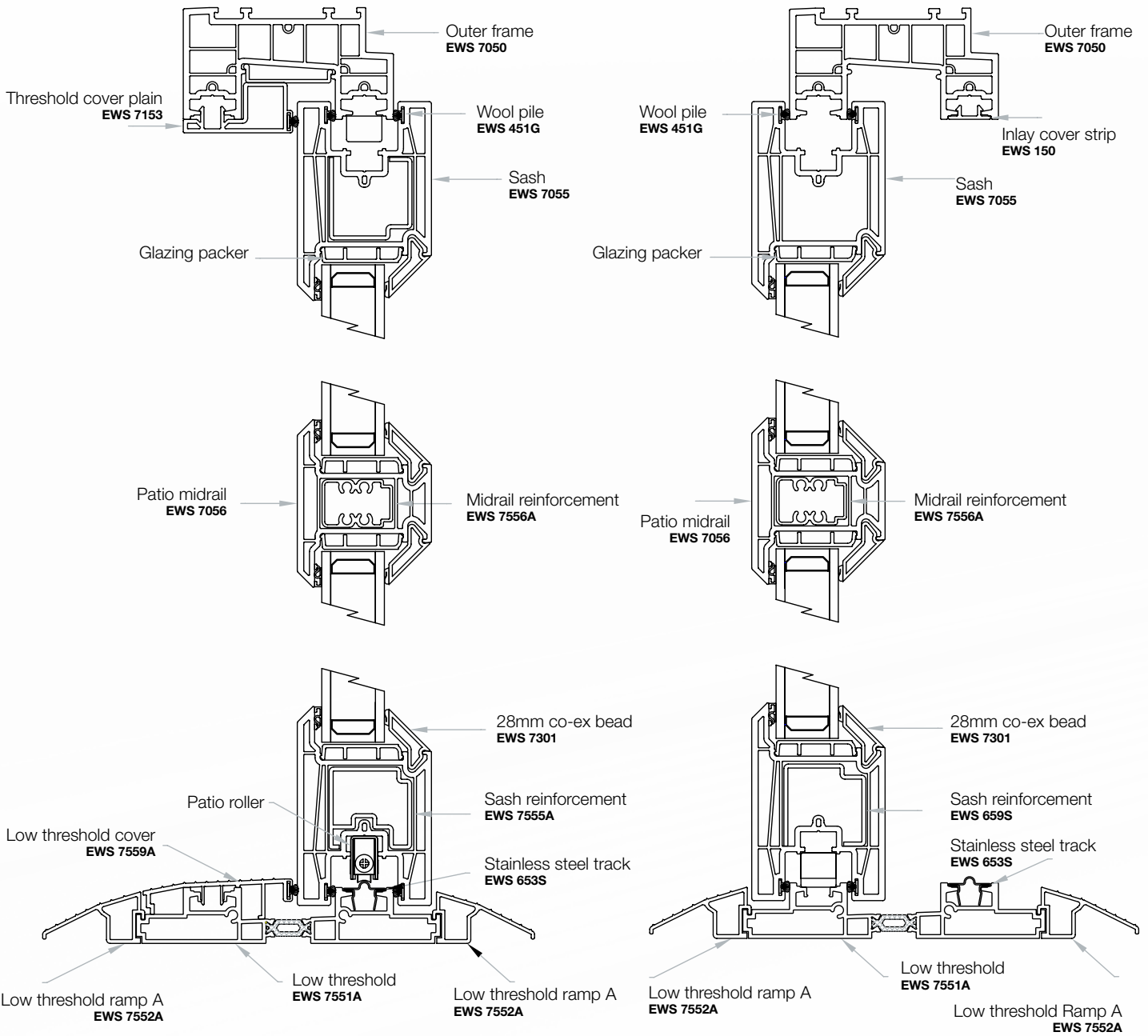
VERTICAL CROSS SECTION THROUGH SLIDING SASH WITH LOW THRESHOLD
