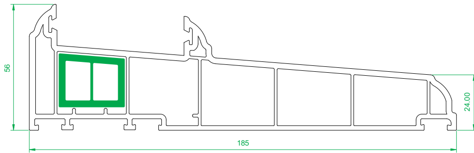
4006 185mm Cill
