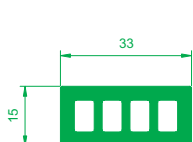
4401 Thermal Insert For 4001 Outer Frame
