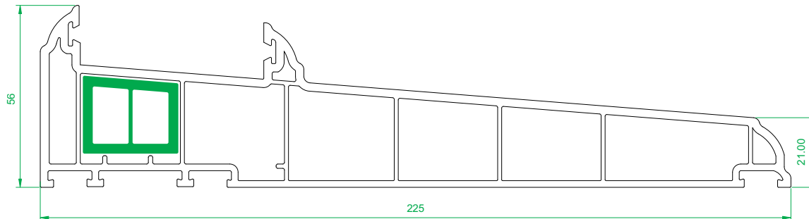
4007 225mm Cill
