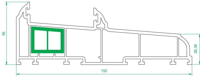
4005 152mm Cill
